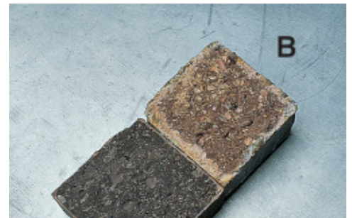
Fig. 2 B - Chloride ion penetration tests (UNI 9944). Specimen A, coated with Mapelastic Zero , appears to be unpenetrated; specimen B, as-is, shows an advanced penetration of several millimetres
